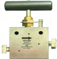
¼" -1" 316 SS 15K-60K TWO-WAY FxF NEEDLE VALVE
